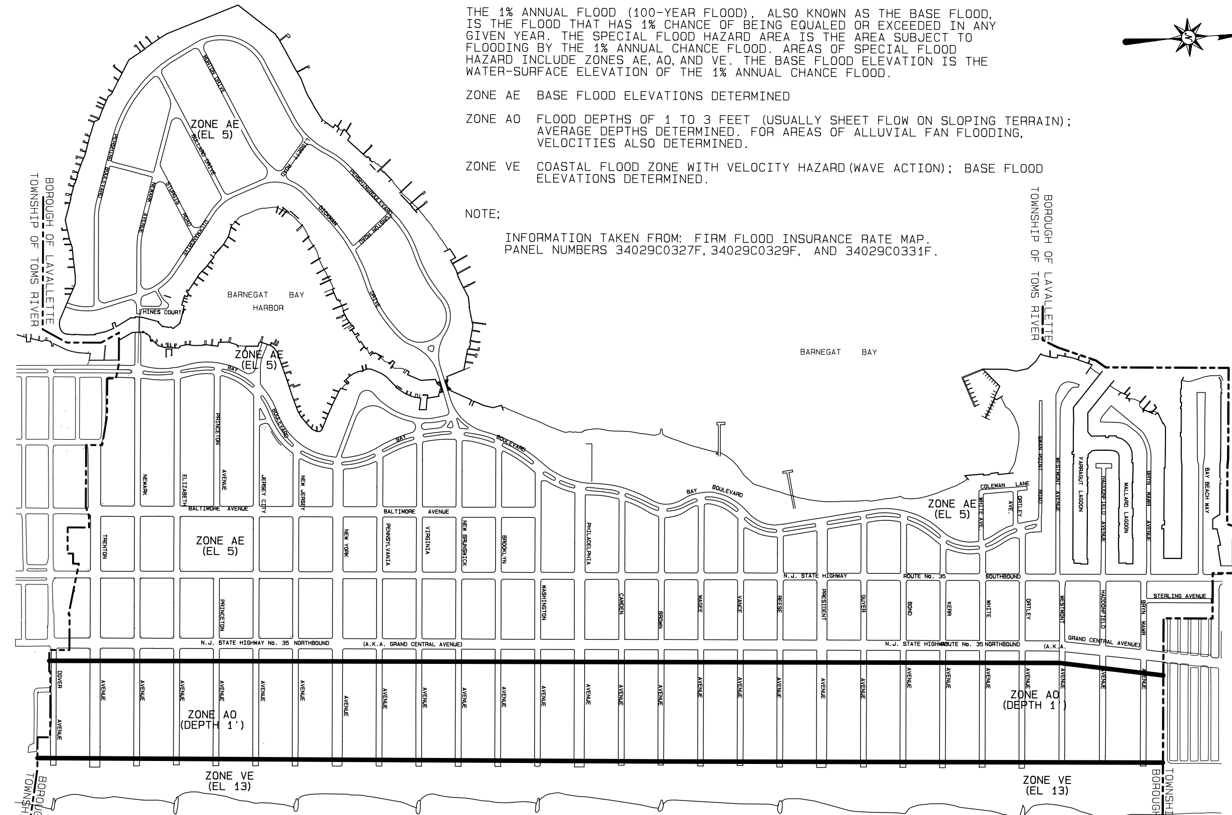
BOROUGH OF LAVALLETTE - FLOOD INSURANCE MAP N.T.S.
